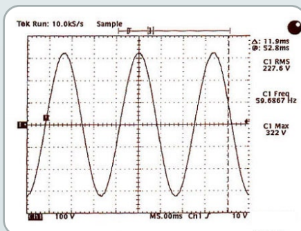
No Load
