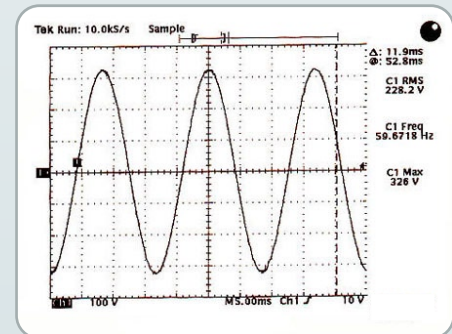
Induction Load
