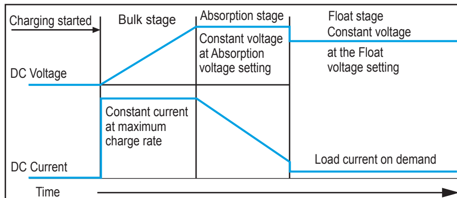
Battery Charging (3 stage charging profile)
